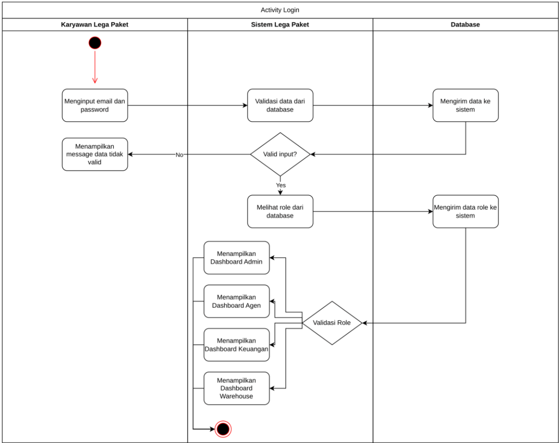
Activity Diagram 1
