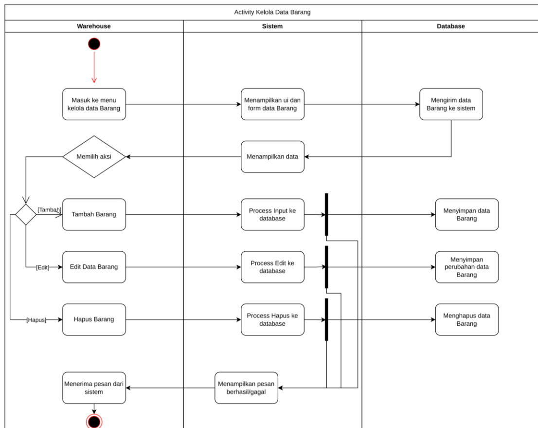
Activity Diagram 10
