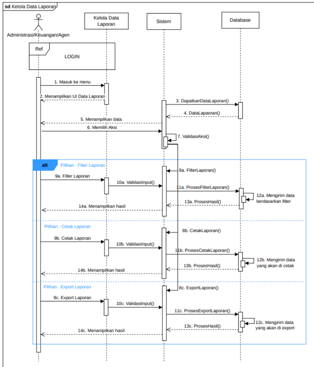
Sequence Diagram 5
