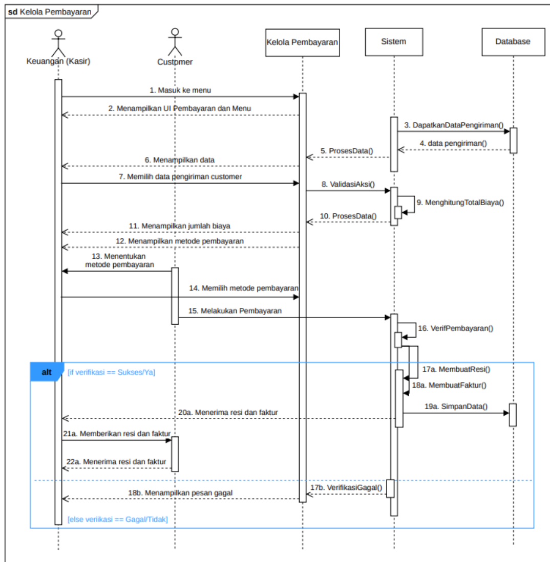
Sequence Diagram 10
