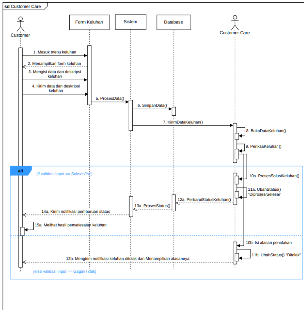
Sequence Diagram 11
