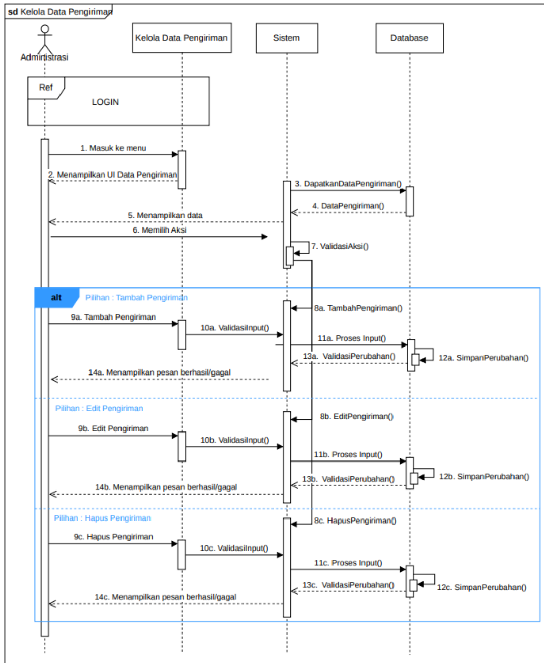
Sequence Diagram 4
