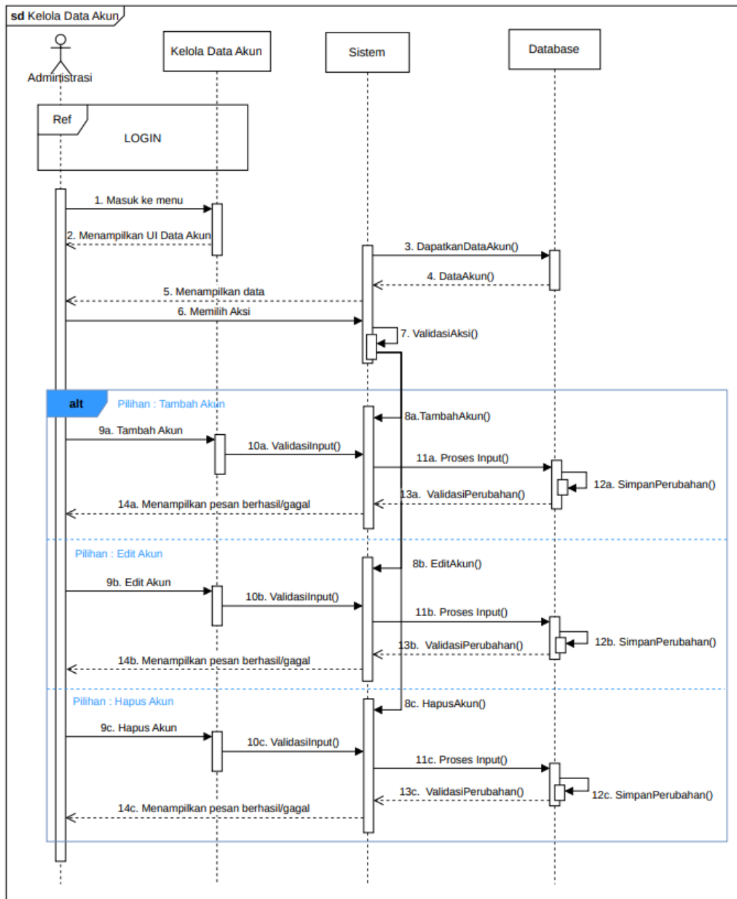
Sequence Diagram 2
