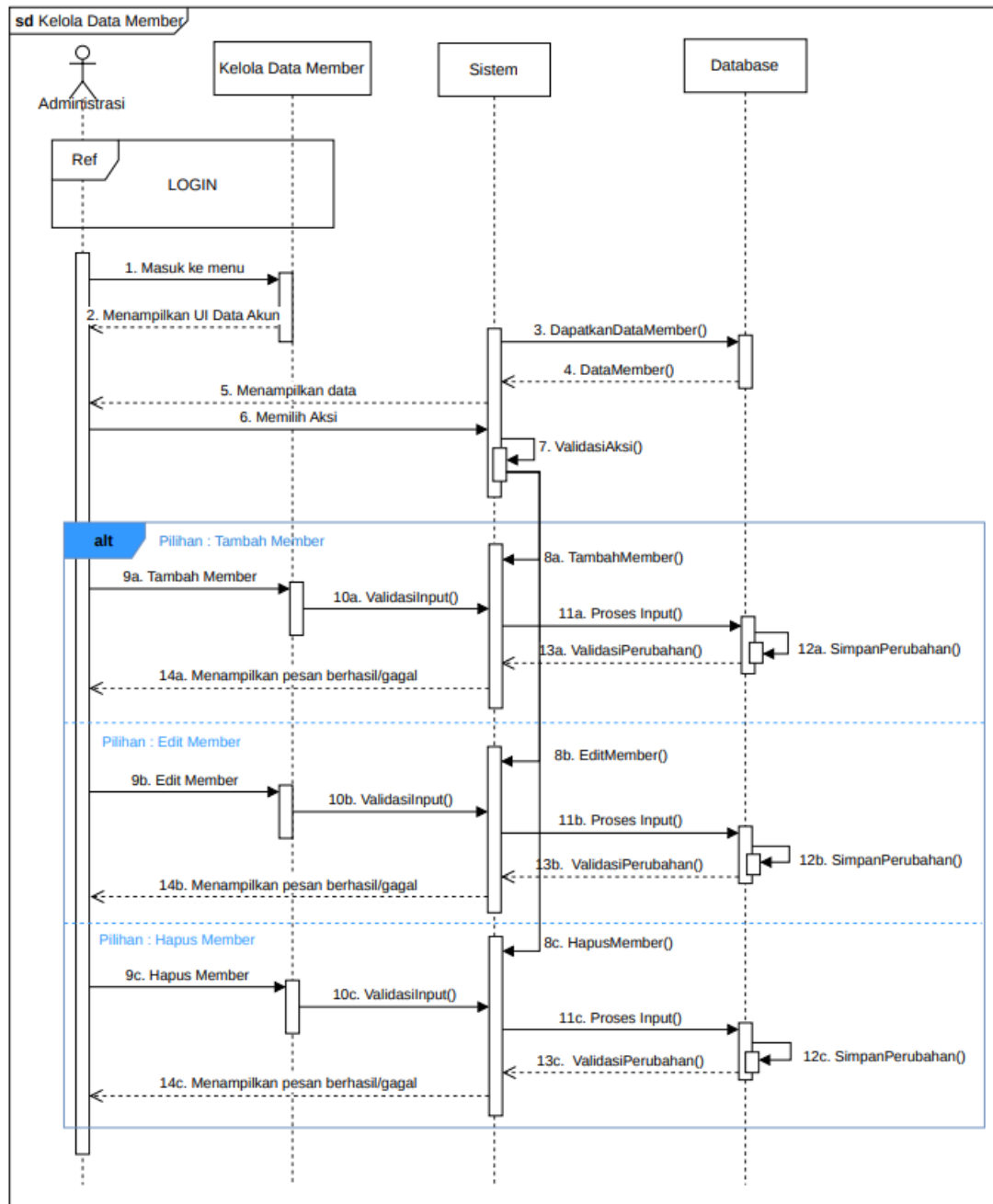
Sequence Diagram 3
