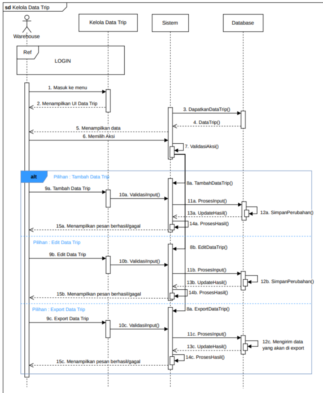
Sequence Diagram 9
