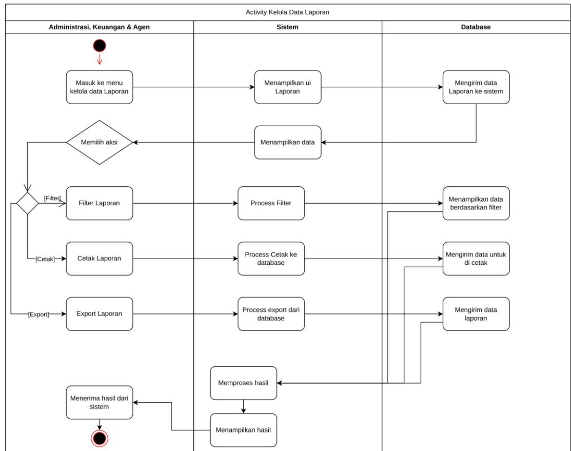
Activity Diagram 5
