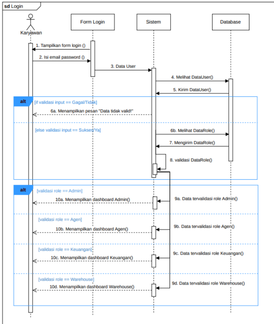
Sequence Diagram 1
