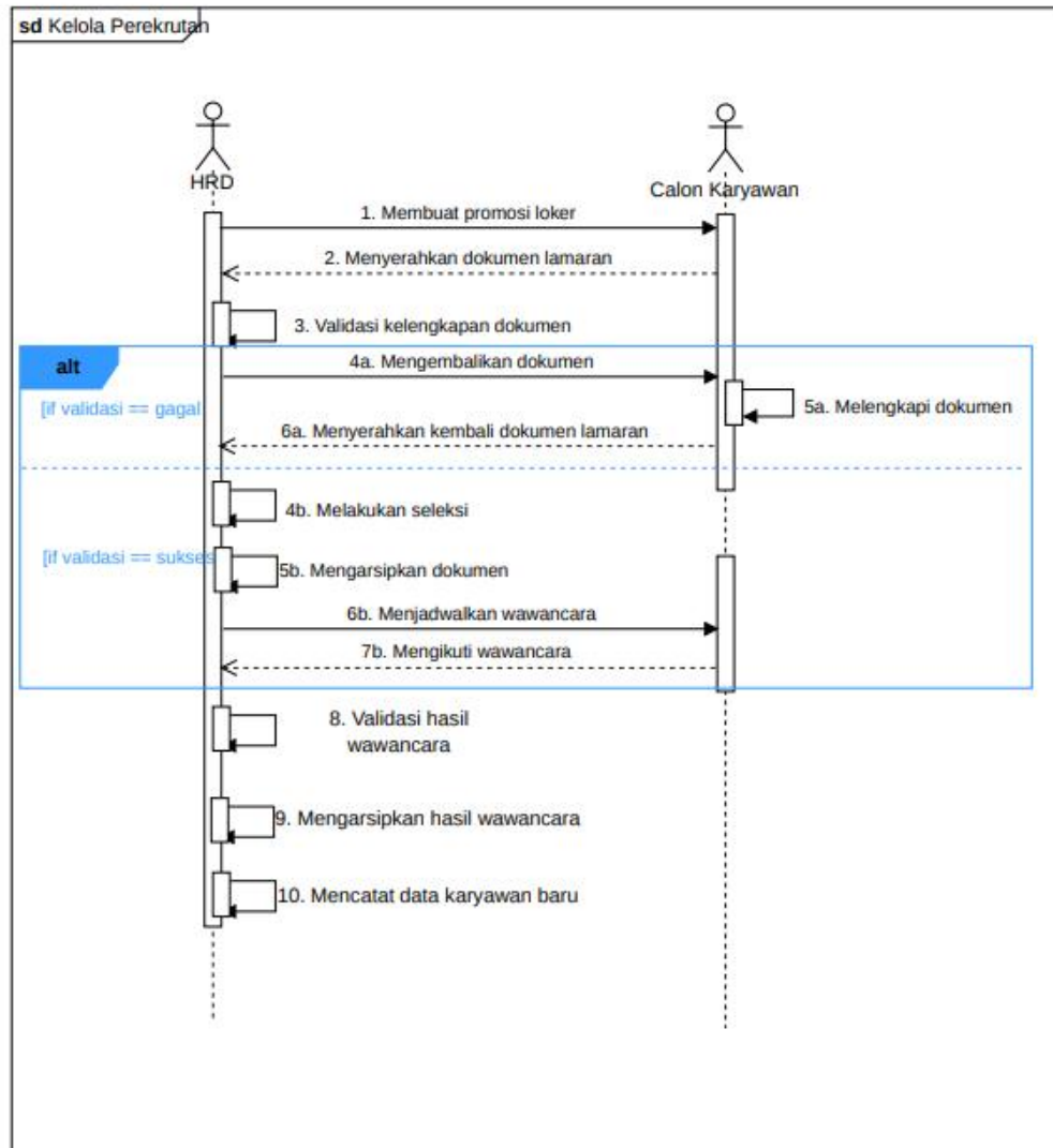
Sequence Diagram 15
