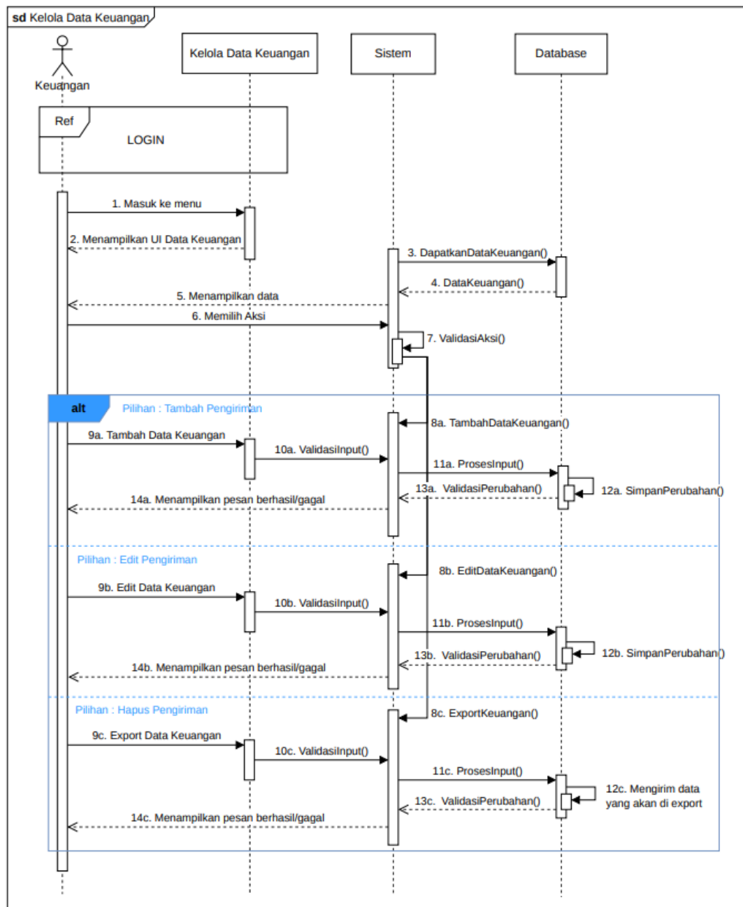
Sequence Diagram 8
