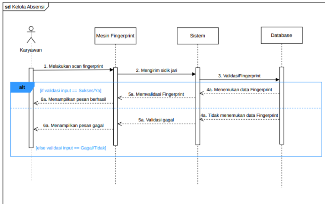
Sequence Diagram 12
