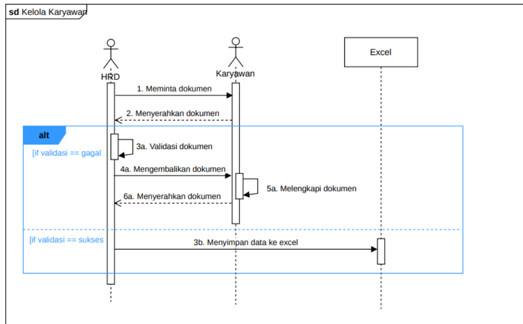
Sequence Diagram 13
