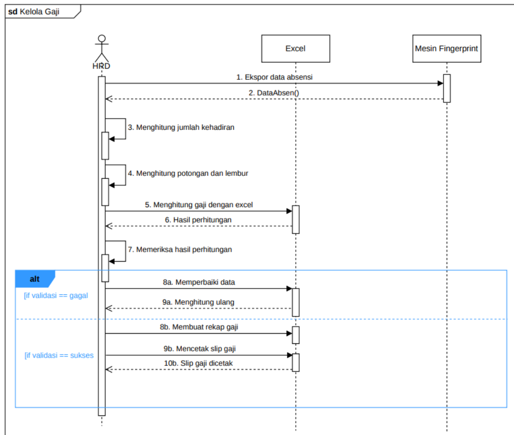
Sequence Diagram 14
