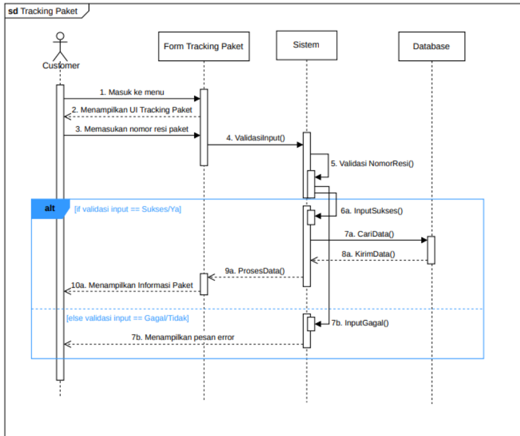
Sequence Diagram 6
