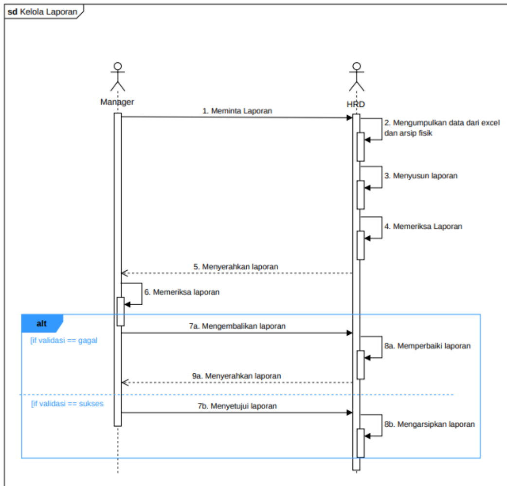
Sequence Diagram 16
