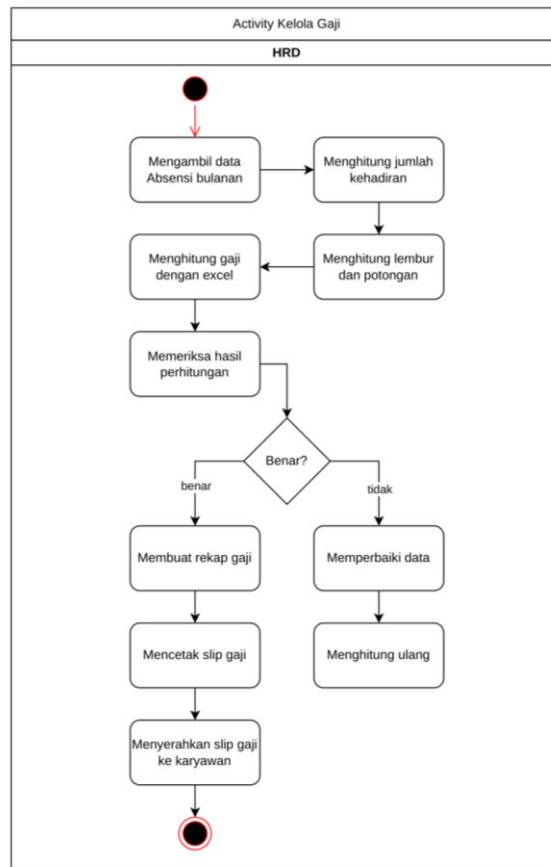
Activity Diagram 8
