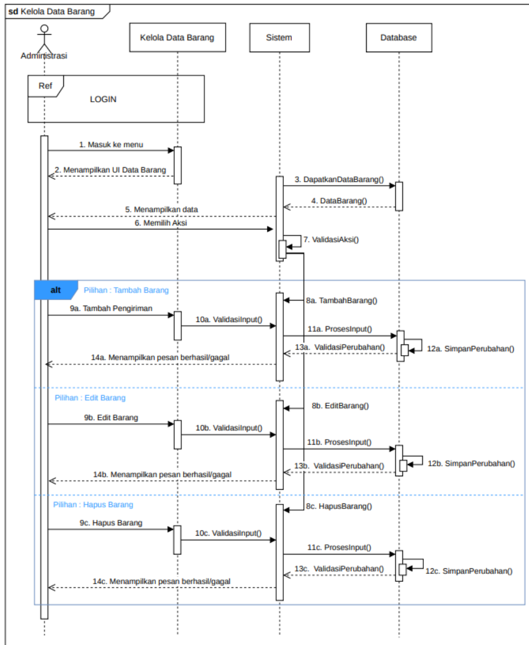
Sequence Diagram 7
